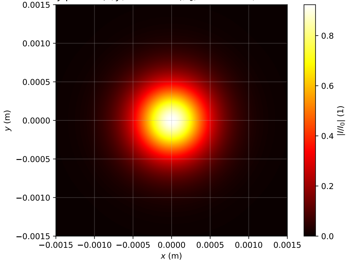
Intensity profile I(x, y, z = 3.742m)/I_0 , \text{Pin}=0.8\text{Pcr} , artificial time
